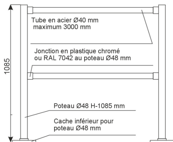
Cloison H-1085 mm:
